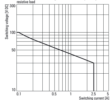
DC Load breaking curve safety output
