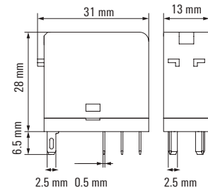
Dimensioned drawing with test button
